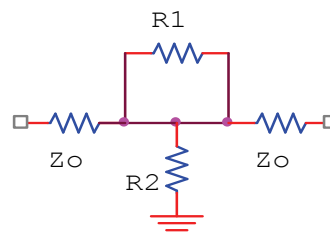
Figure 4: Bridged-Tee Attenuator
