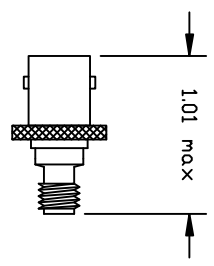
BNC Female - SMA Female Model 412-442-011
