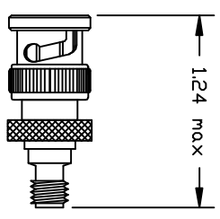
BNC Male - SMA Female Model 412-441-012
