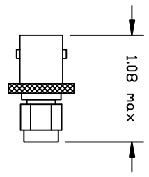
BNC Female - SMA Male Model 411-442-017
